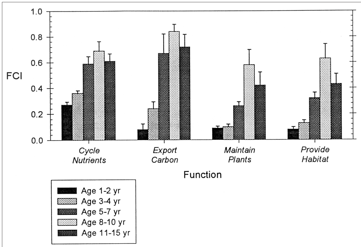
Figure 1. Average functional capacity index (FCI) values for four functions at 49 forested wetland sites of various ages since abandonment from agriculture or restoration by planting trees. Sites were grouped by age classes indicated in the legend. Error bars indicate 1 standard error of the mean.
